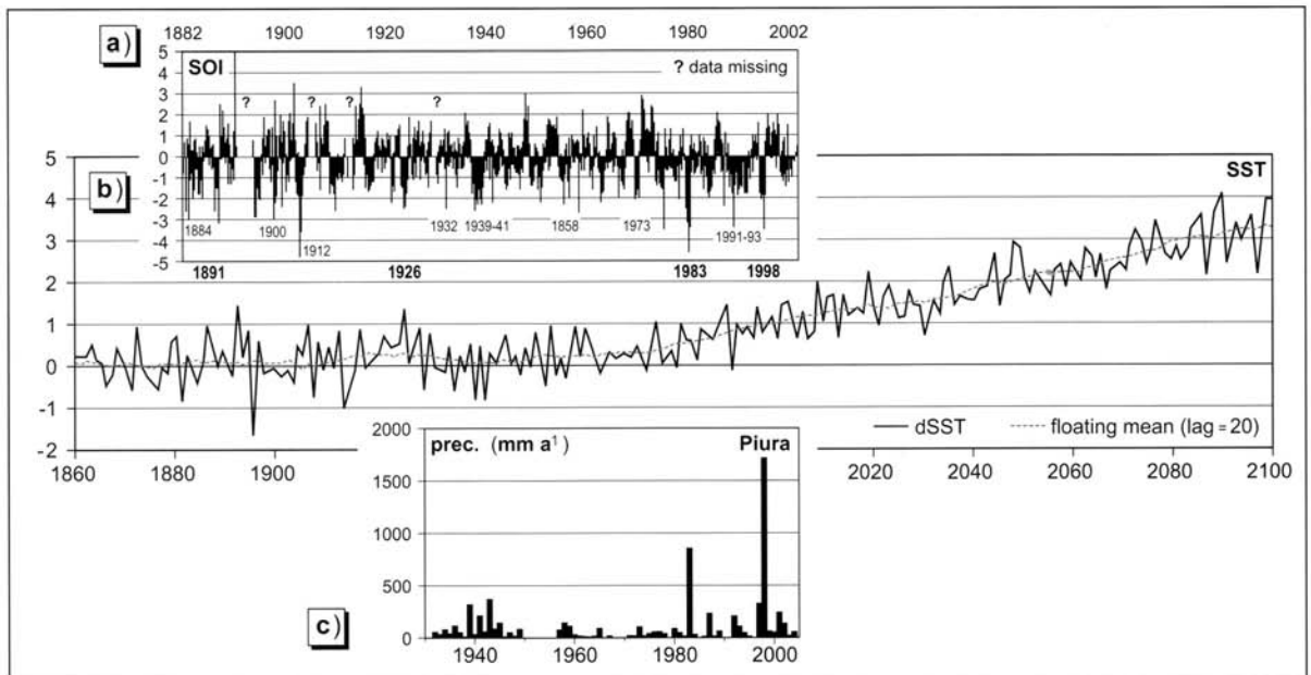
Fig. 6: Indicator values for past and future El Niño activity: (a) Southern oscillation index (SOI) between 1882 and the present (source: http://sevilleta.unm.edu/data/contents/SEV016/ ), (b) development of sea surface temperatures (SST) between 1860 and the present and scenario of a future increase based on coupled ocean-atmosphere models (source: BENDIX et al. 2000) and (c) annual rainfall amounts at Piura from 1932 until now (Data: Proyecto Chira y Piura)
