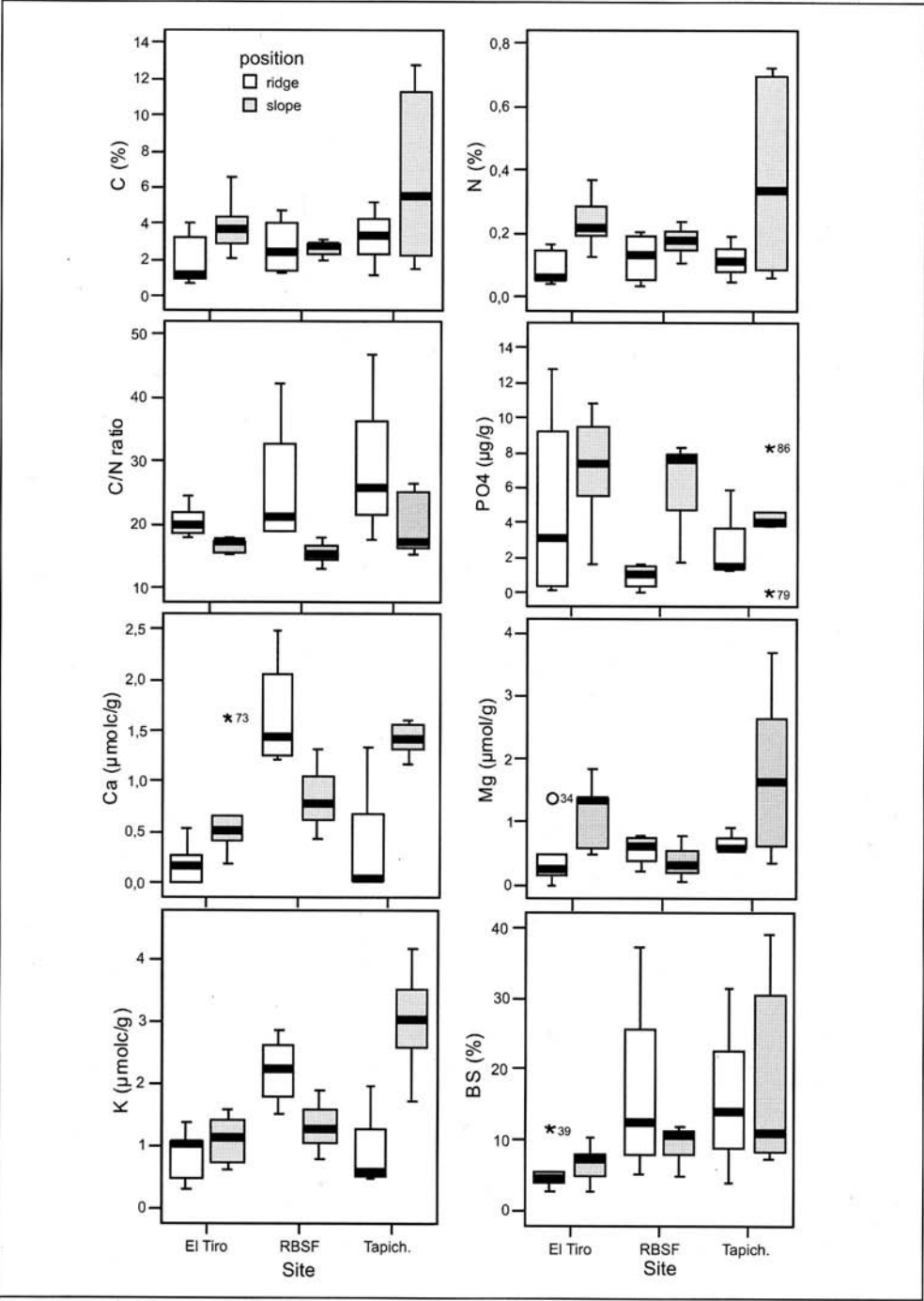
FIG. 5. Soil chemical parameters in the Ah horizons [org. Carbon (C), total nitrogen (N), C/N ratio, citric acid extractable \text{PO}_4^{3-} ( \text{PO}_4 ), exchangeable base cations (K, Ca, Mg) and base saturation (BS)].
